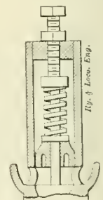
SAFETY VALVE.
